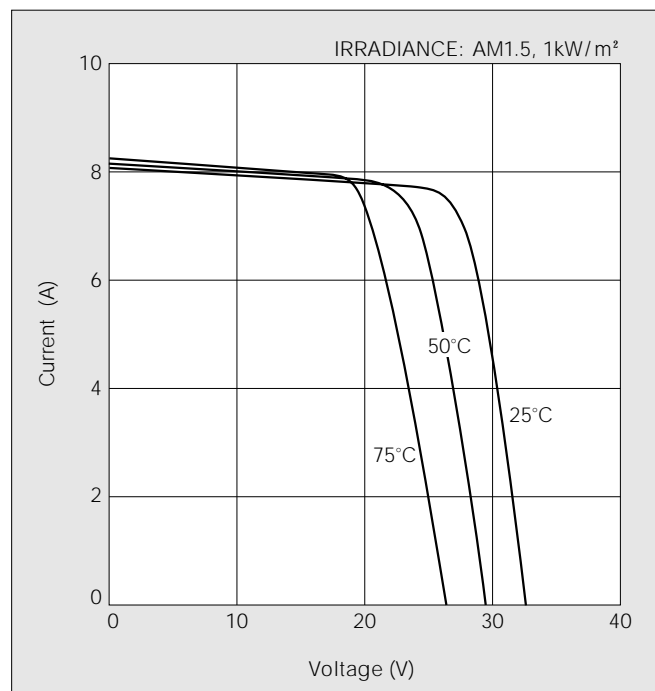
Current-Voltage characteristics of Photovoltaic Module KC190GT at various cell temperatures
