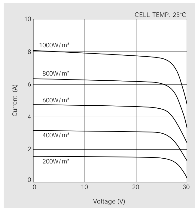
Current-Voltage characteristics of Photovoltaic Module KC190GT at various irradiance levels
